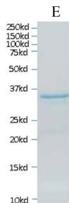
E: SARS-CoV-2/Wuhan/2019 Envelope
